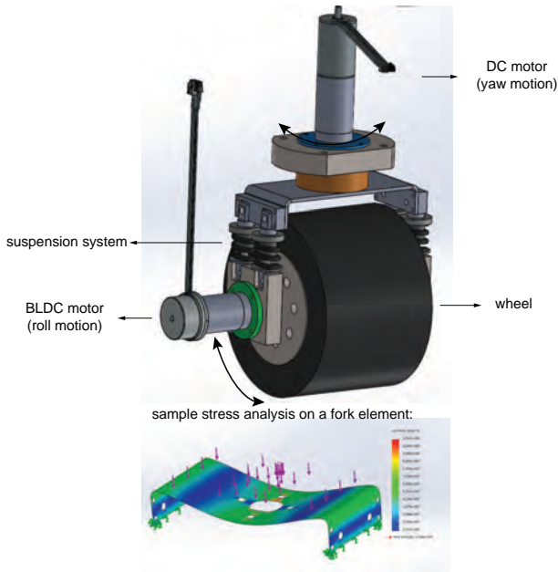
Fig. 3. The omni-directional wheel - a key element of a robot
