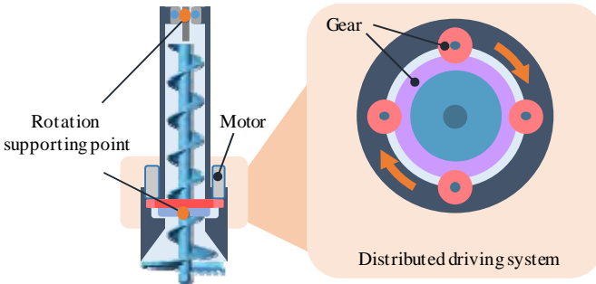
Figure 5. Concept of the distributed driving system.
