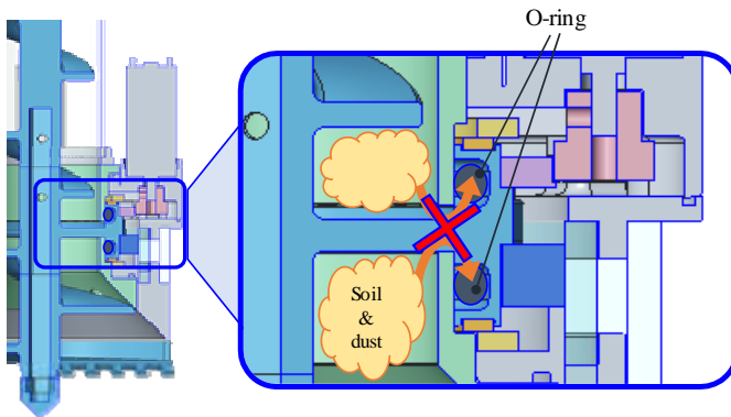
Figure 7. Overview of dustproofing system.
