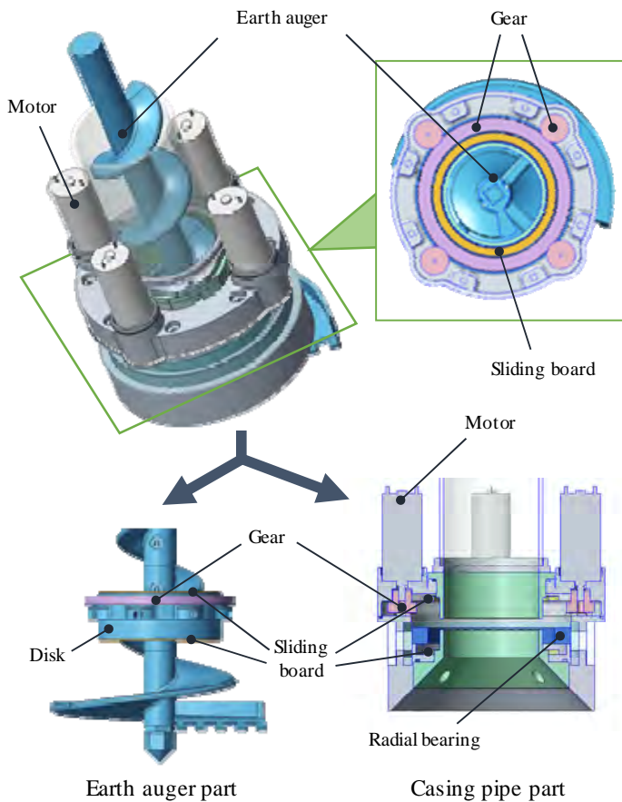
Figure 6. Prototype of the distributed driving system.
