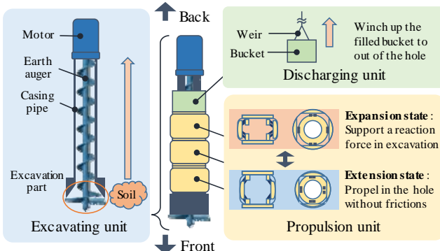
Figure 1. Overview of the LEAVO.
