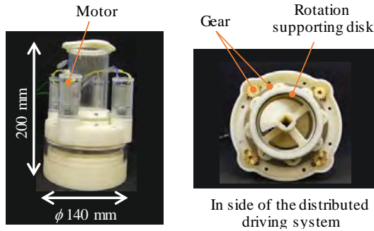
Figure 8. Appearance of the distributed driving system prototype.
