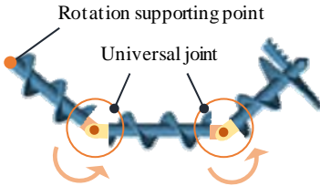
Figure 3. Flexible auger.
