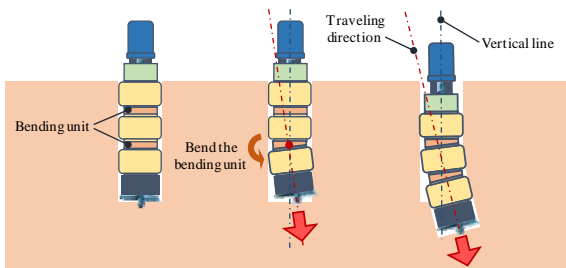
Figure 2. Overview of curved excavation.
