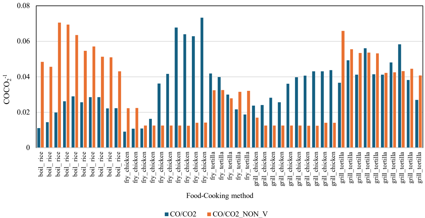
Figure 10. CO/CO 2 -1 ratio by cooking method.
