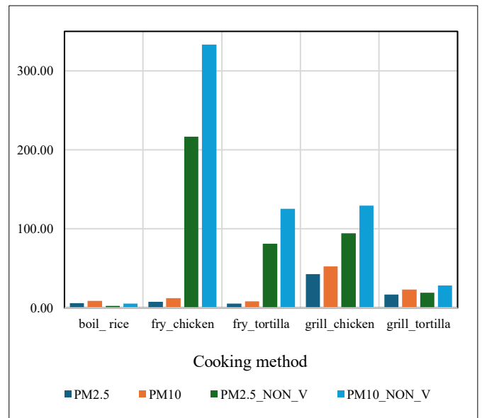
Figure 11. Influence of the cooking method on the behavior of particulate matter under normal ventilation conditions, minimum ventilation conditions (NON_V).
